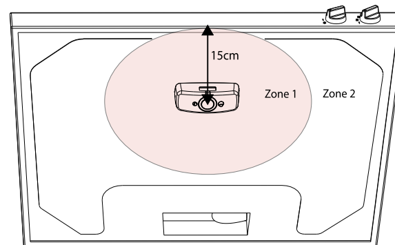
Zone 1: above the central point of the cooker (max. 15 cm tolerance to the side).
